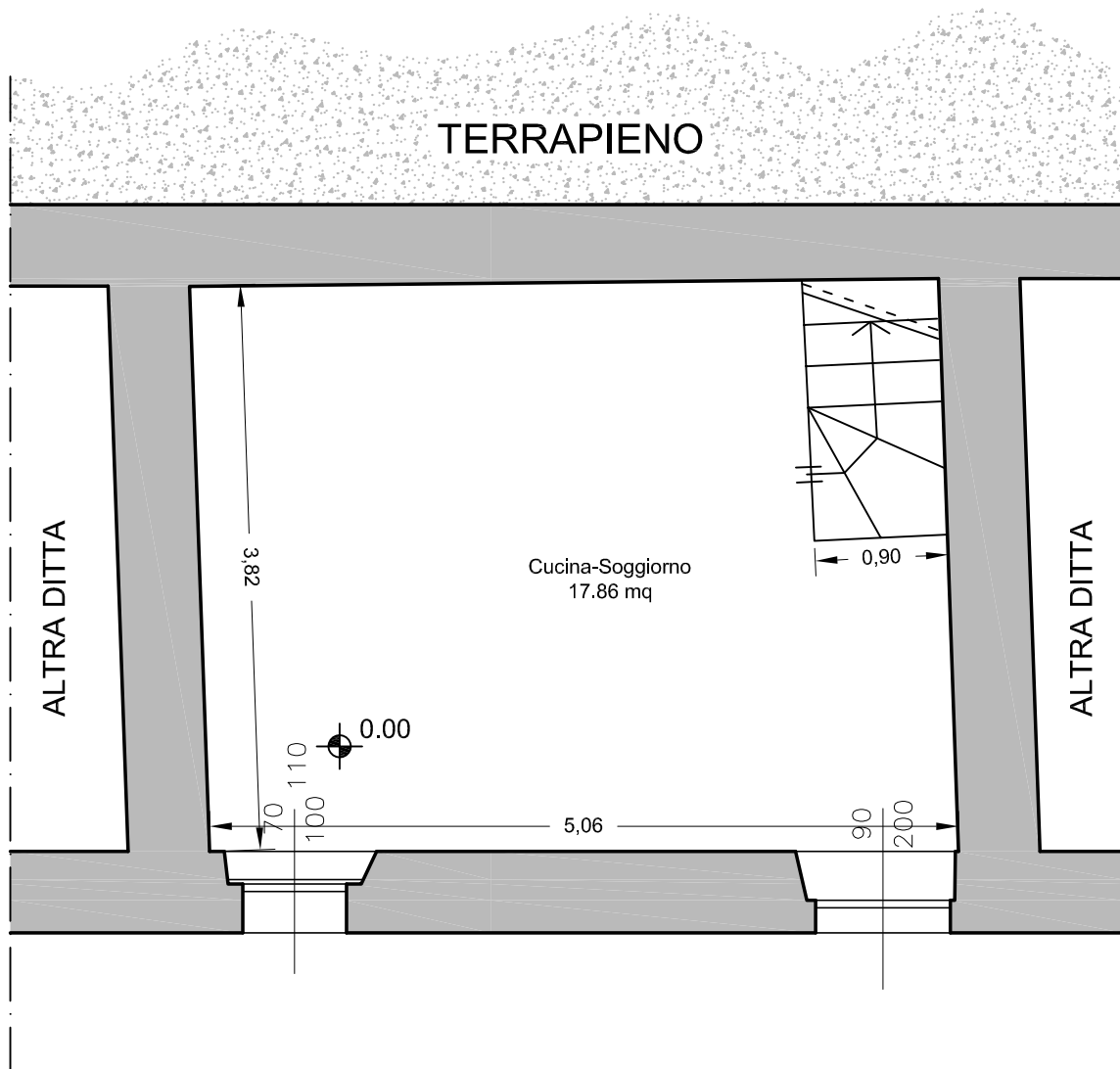
PIANO TERRA
